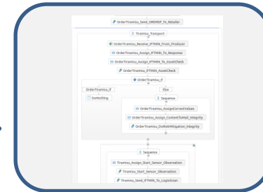
BPEL Workflow
